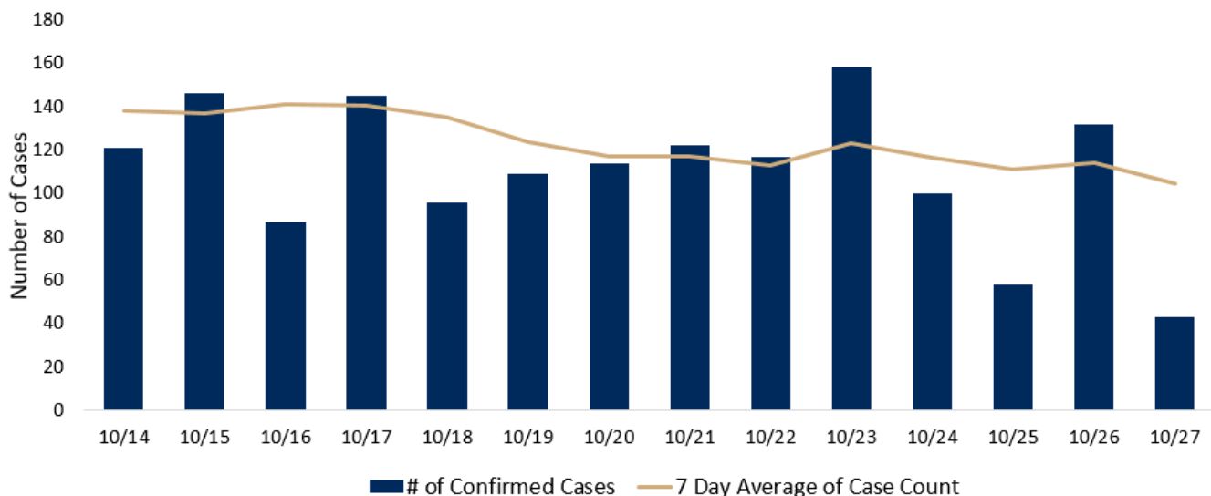
Daily Confirmed Case Count in Past 14 Days (October 14-October 27)
