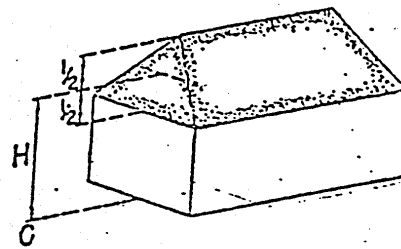
HIP ROOF
